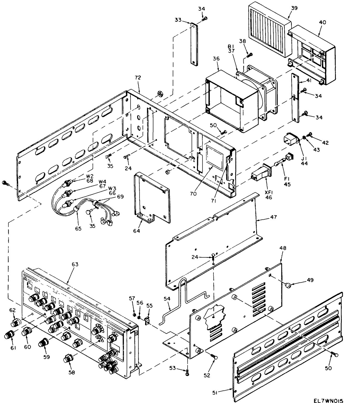
Figure 1. Calibrator, AC 0-1804/USM-410(V) (Sheet 2 of 4).
