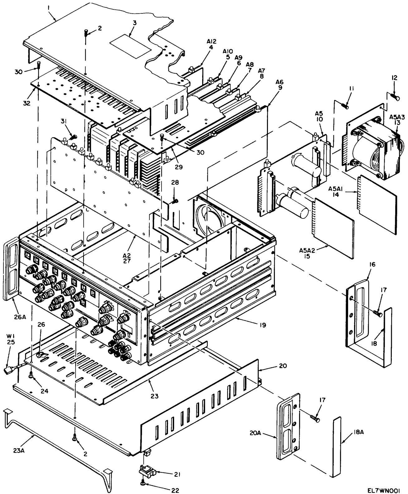
Figure 1. Calibrator, AC 0-1804/USM-410(V) (Sheet 1 of 4).
