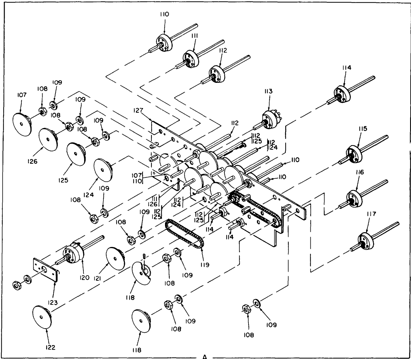
Figure 1. Calibrator, AC 0-1804/USM(V) (Sheet 4 of 4).
