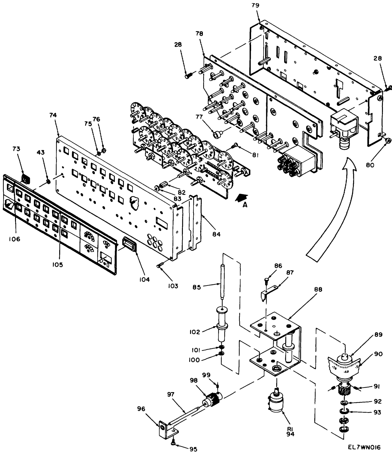
Figure 1. Calibrator, AC 0-1804/USM-410(V) (Sheet 3 of 4).
